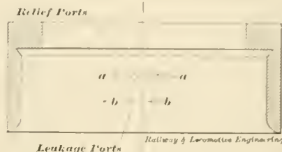
FIG. 5. PORTS IN BUSHING.
